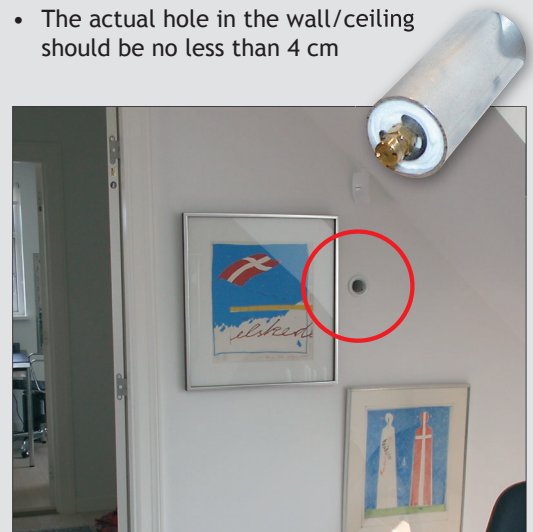
Horizontal installation
